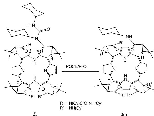
Scheme 2. Access to chiorporphyrin 2m with mono- N -substituted amide groups
