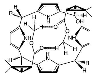
Figure 3. Conformation of an \alpha,\beta,\alpha,\beta substituted tetrapyrrole intermediate, preorganised by weak C–H...O hydrogen bonds between methyl ester substituents, which leads to facile cyclisation to the porphyrinogen. For the sake of clarity, only the H-bonding pattern on the top face is shown, and each of the two meso substituents on the bottom face is abbreviated as R
