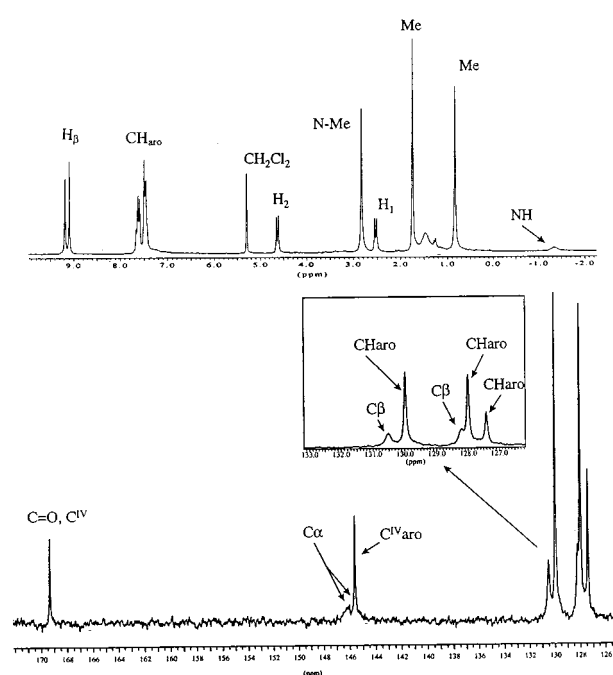
Figure 2. ^1\text{H} (top) and ^{13}\text{C} (bottom) NMR spectra of tetra- N -methyl- N -phenylchiroporphyrin 2j
