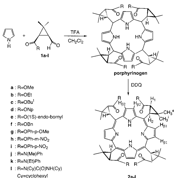
Scheme 1. One-pot, two-step synthesis of chiorporphyrins 2a–l
