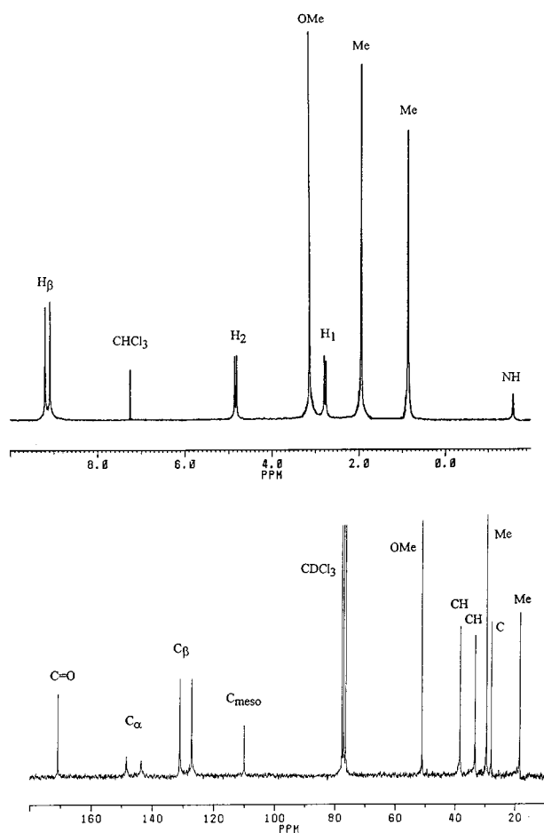
Figure 1. ^1\text{H} (top) and ^{13}\text{C} (bottom) NMR spectra of tetramethyl-chiroporphyrin 2a
